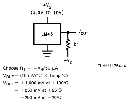
FIGURE 2. Full-Range Centigrade Temperature Sensor ( -20^\circ\text{C} to +100^\circ\text{C} )
