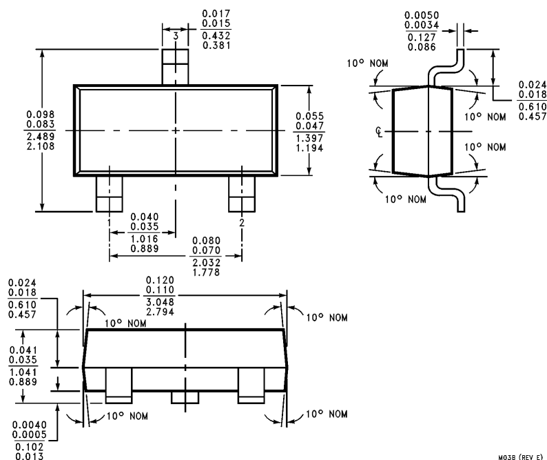
SOT-23 Molded Small Outline Transistor Package (M3) Order Number LM45BIM3, LM45BIM3X, LM45CIM3 or LM45CIM3X NS Package Number M03B (JEDEC Registration TO-236AB)
